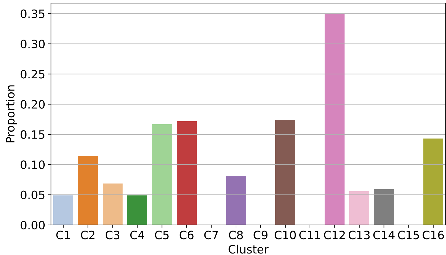
Immunodeficiency (i.e auto-immune disease) proportion by cluster
